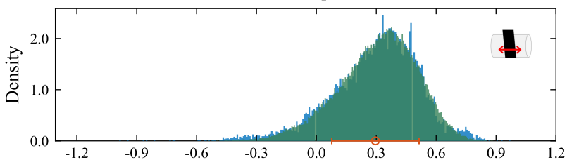
Error, tape lateral movement
