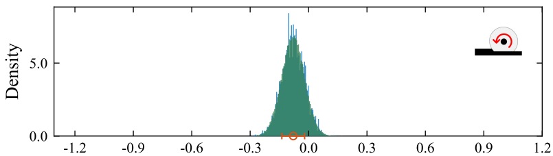
Error, tape width after compaction
