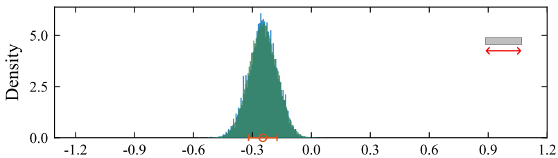
Error, tape width before compaction
